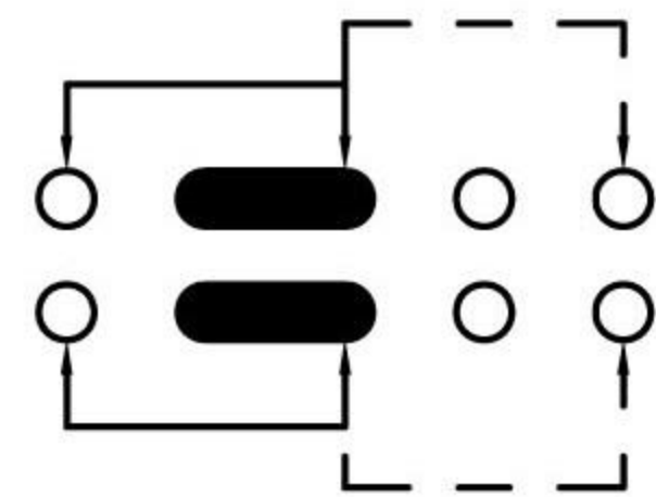
SCHEMATIC (NON-SHORTING)
